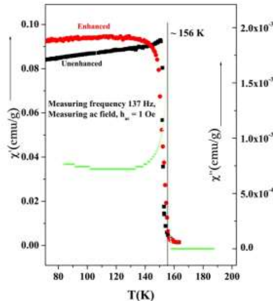
Figure 5: \chi'(T) in the presence of enhancing field, and that in the absence of enhancing field (Left y-axis); \chi''(T) in the absence of enhancing field (Right y-axis).
